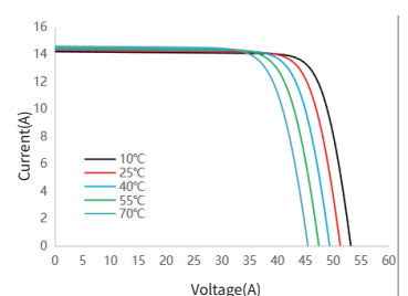
I-V Curve at Different Temperature SS8-72HD-575N
