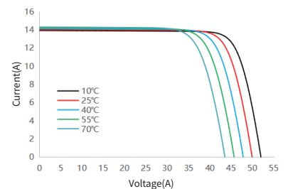
I-V Curve at Different Temperature SS8-72HS -550M
